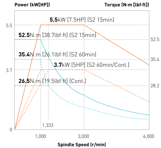
BMT55 6,000 rpm
